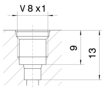
Fig. 6: Profiled bore for V 8 x 1 thread
