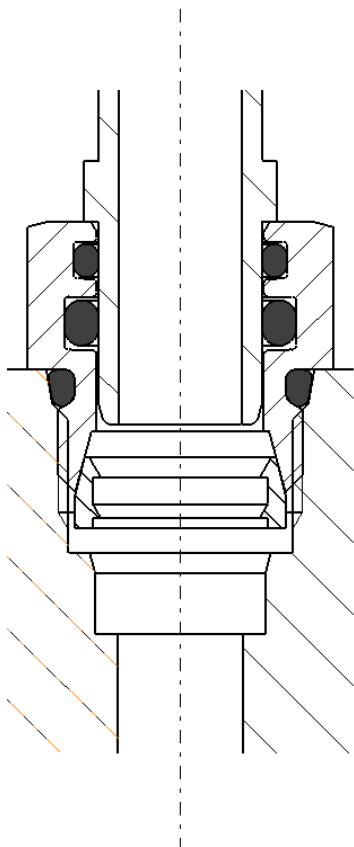
Fig. 25: Schematic diagram for a male gauge
