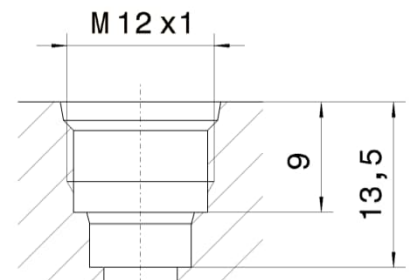
Fig. 5: Profiled bore for M 12 x 1 thread
