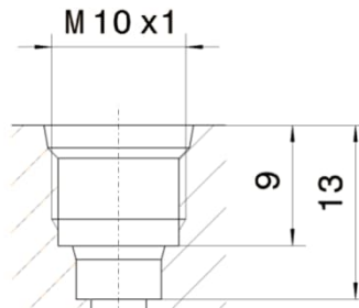
Fig. 4: Profiled bore for M 10 x 1 thread
