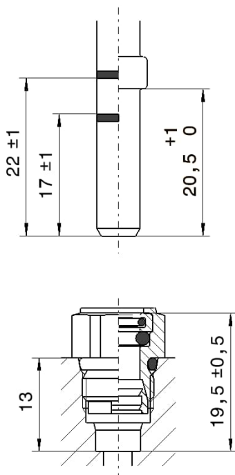
Fig. 21: Push-in depths and dimensions NS 4 and NS 6
