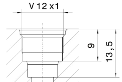
Fig. 8: Profiled bore for V 12 x 1 thread
