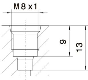
Fig. 3: Profiled bore for M 8 x 1 thread
