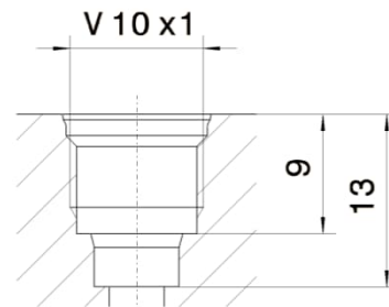
Fig. 7: Profiled bore for V 10 x 1 thread
