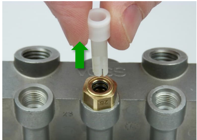
Fig. 16: Pulling out the assembly plug
